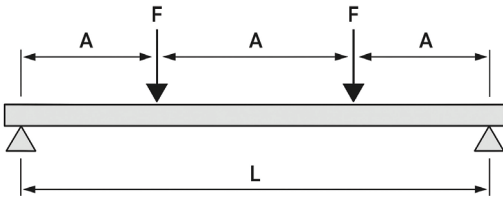
L = length, A = equal distances, F = load point
